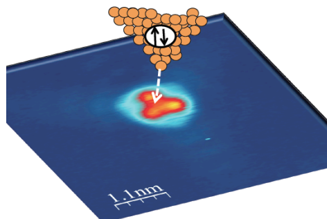
Spatial map of a low-energy bound state around a Fe nanoisland on superconducting Pb and sketch of STM experiment.
